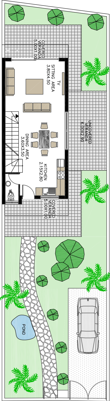
GROUND FLOOR HOUSE TYPE G
