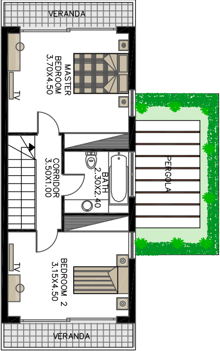
FIRST FLOOR HOUSE TYPE G
