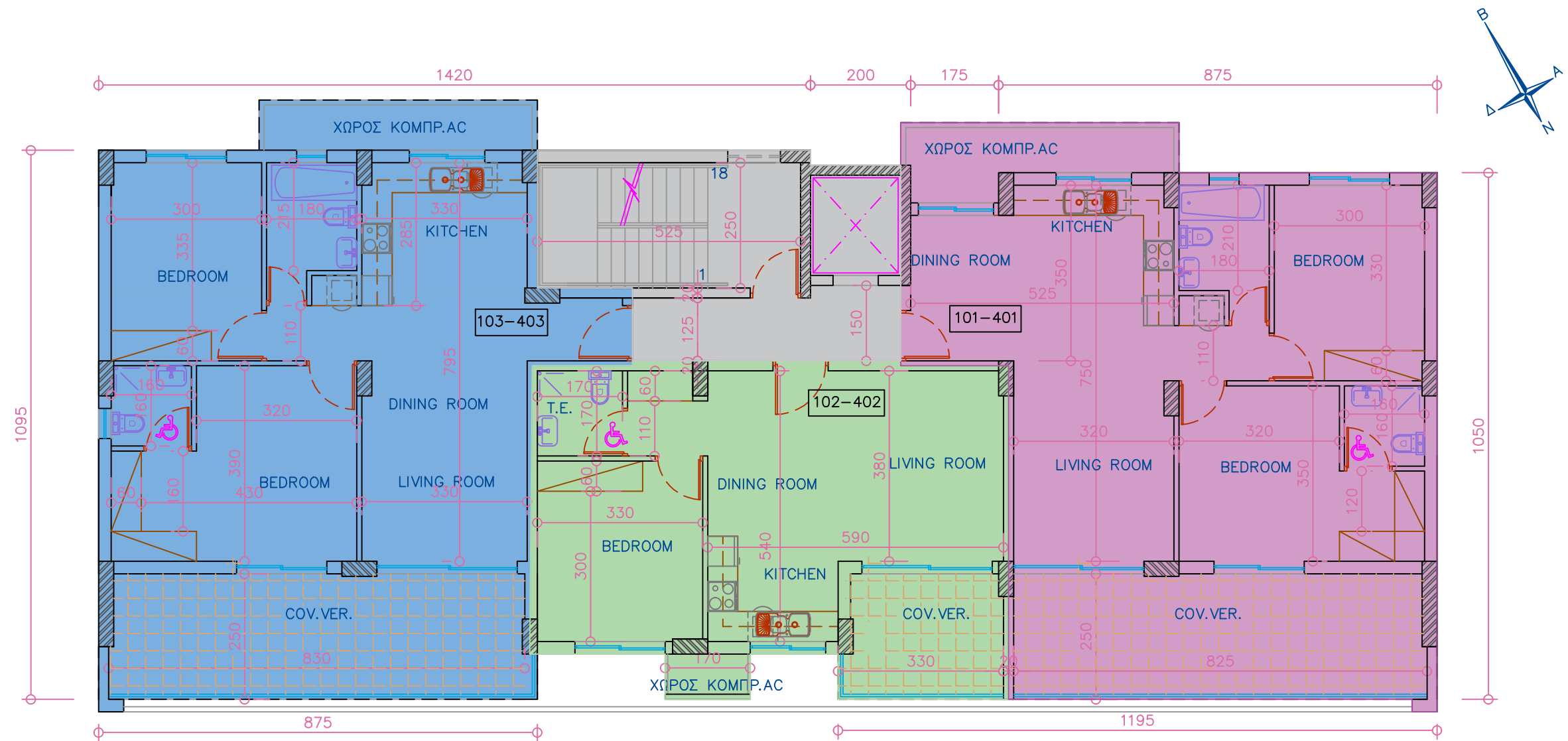
ΚΑΤΟΨΗ 10Τ-40Υ ΟΡΟΦΟΤ BLOCK A
