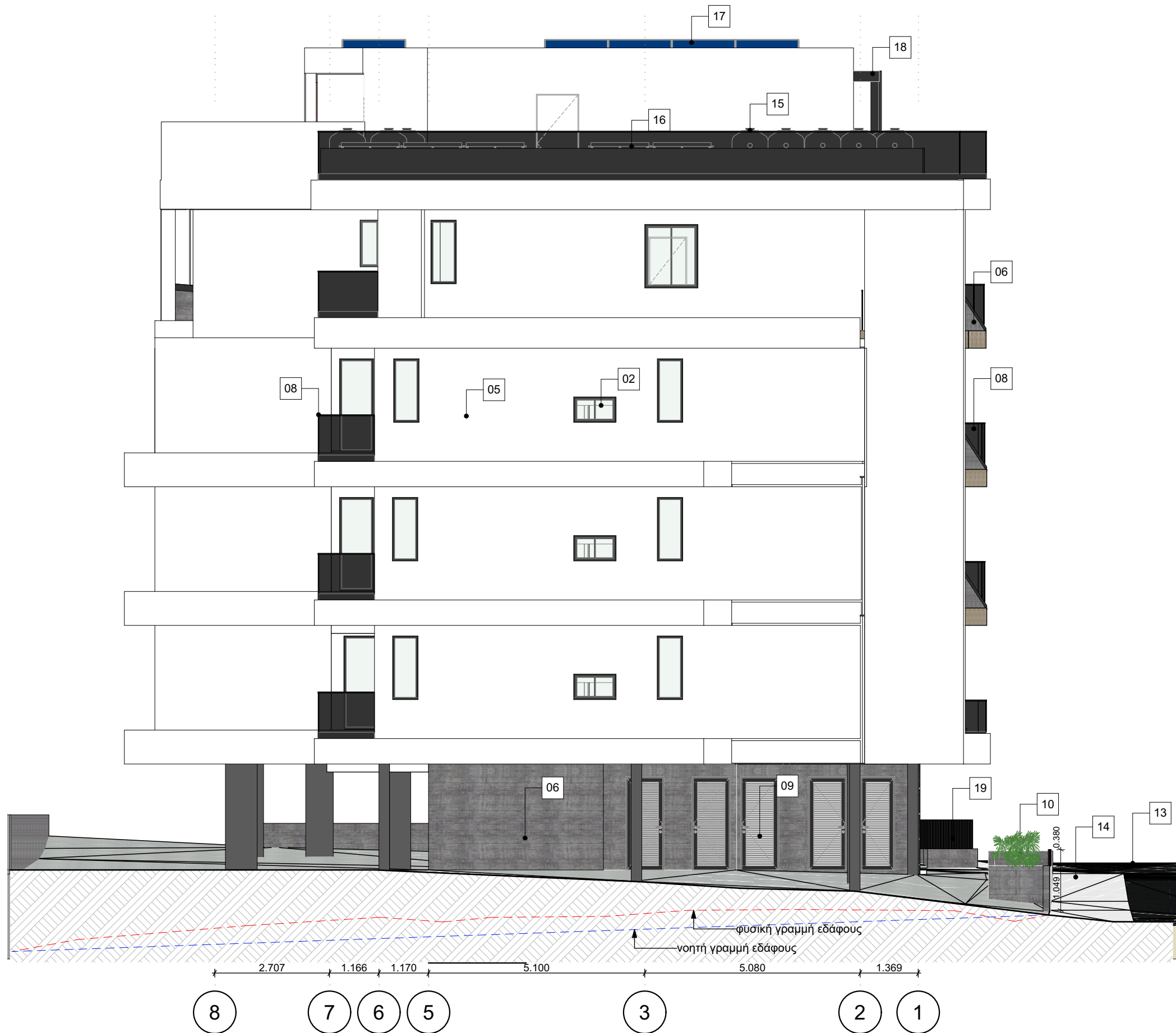
North Elevation
