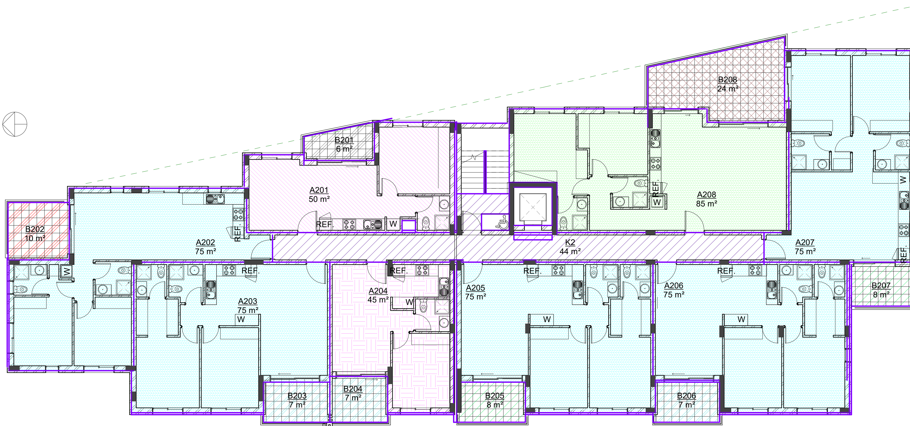
2 Second Floor 1 : 100
