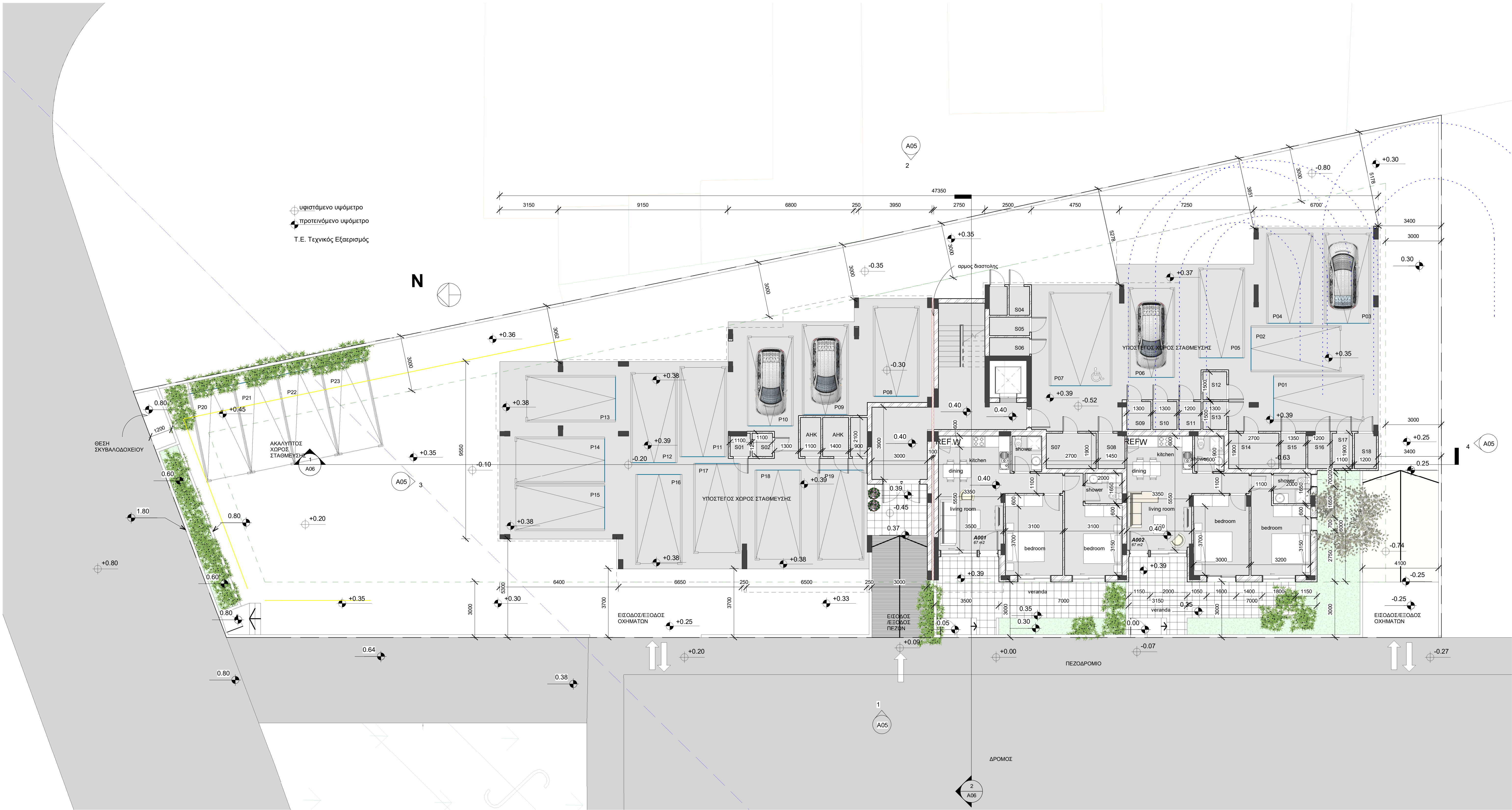
1 Ground Floor 1:100
