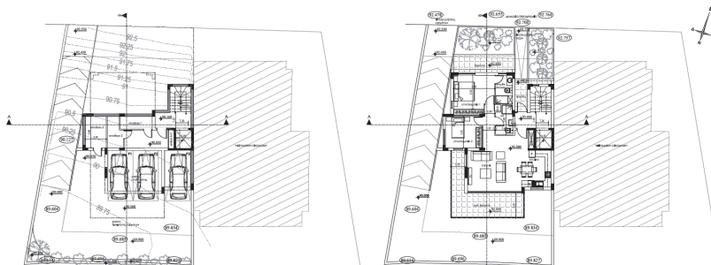
SEMI-BASEMENT FLOOR
