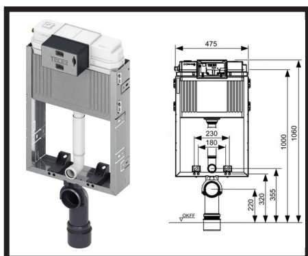
TECE Unicistern 13cm brick wall
