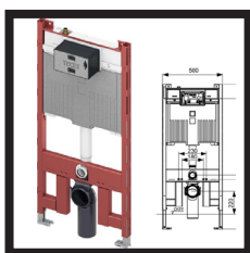
TECE Unicistern 13cm brick wall
