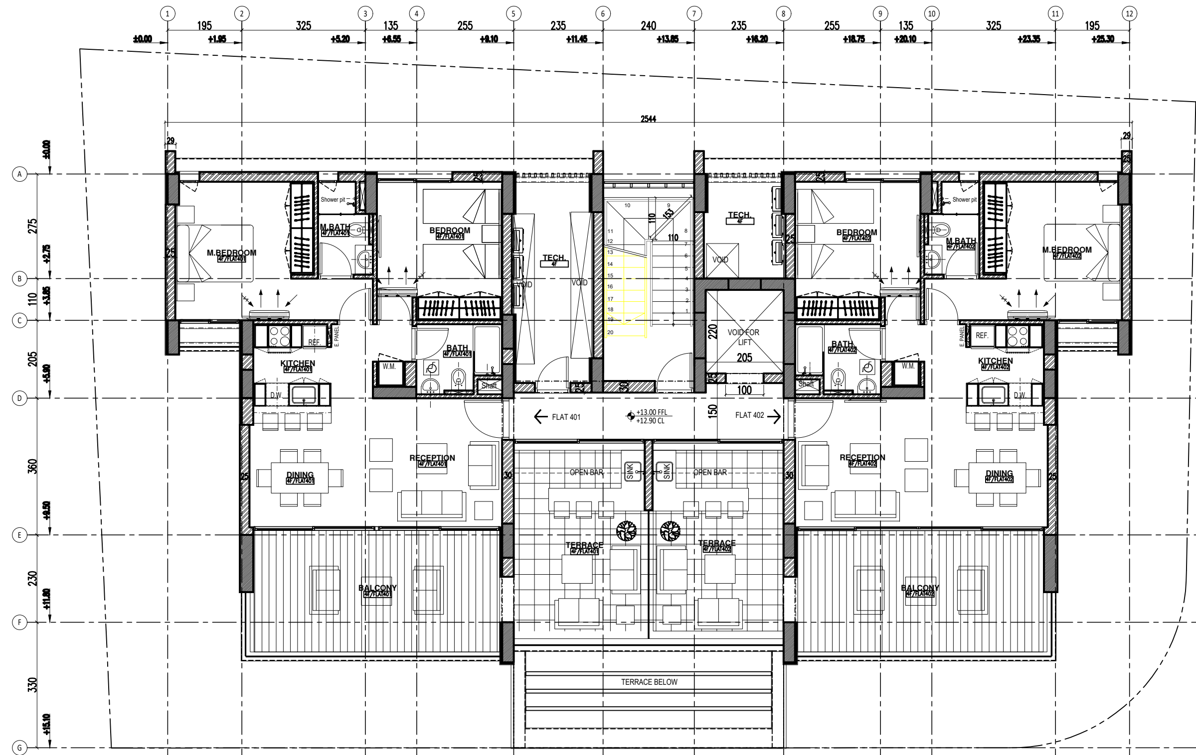
FOURTH FLOOR
