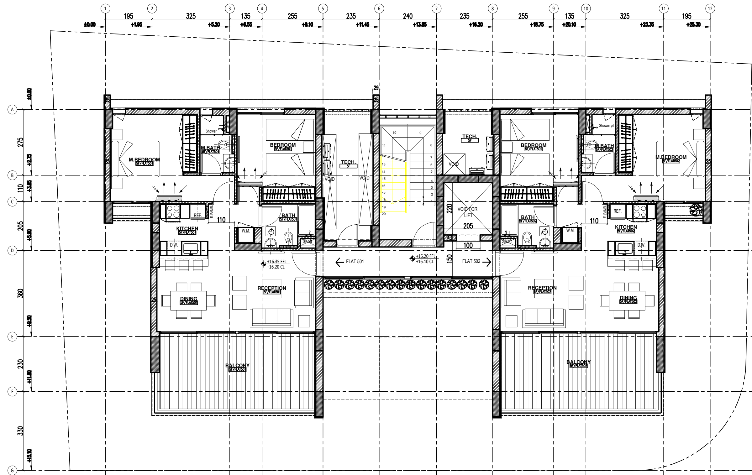
FIFTH FLOOR
