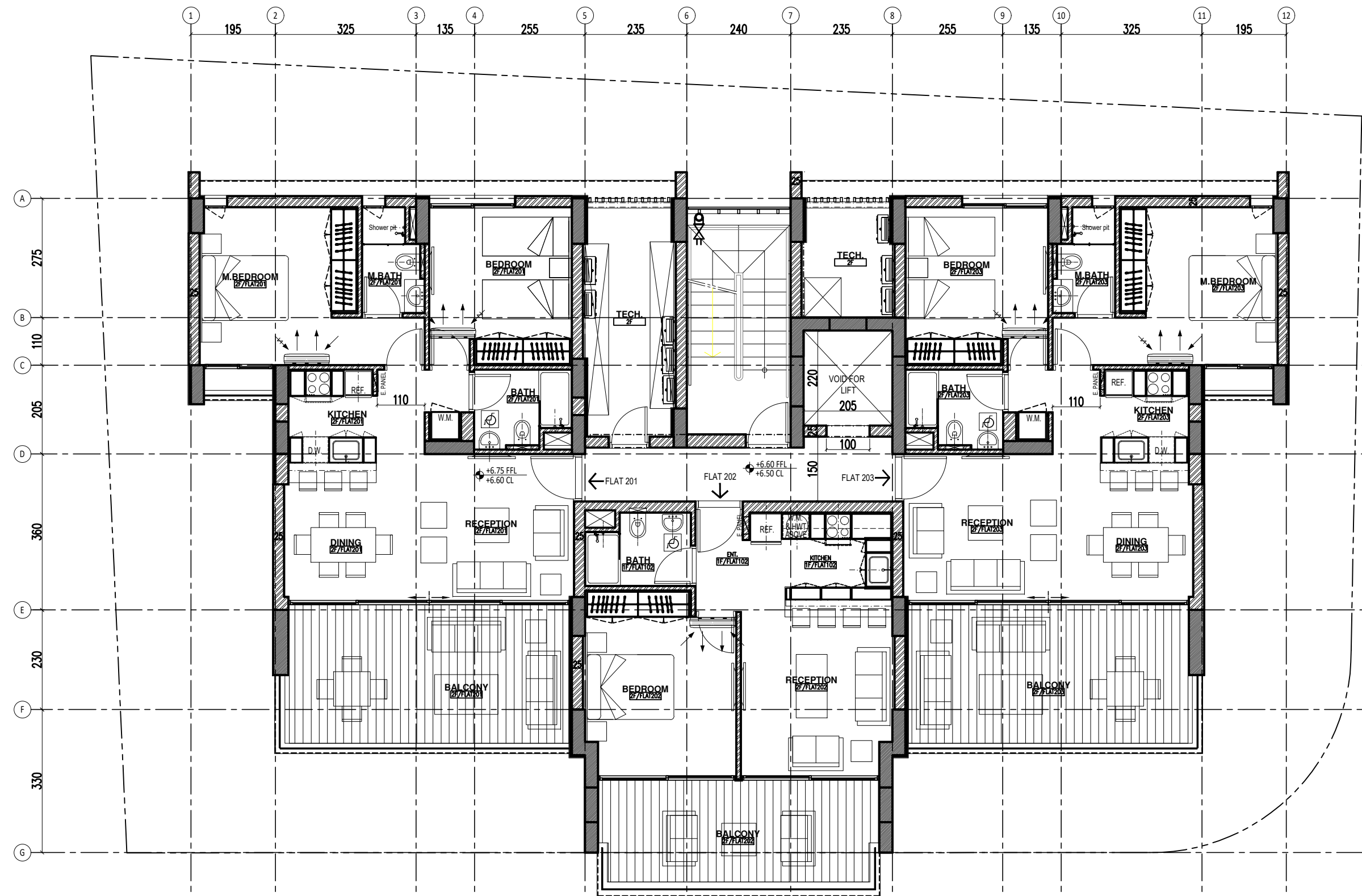
SECOND FLOOR
