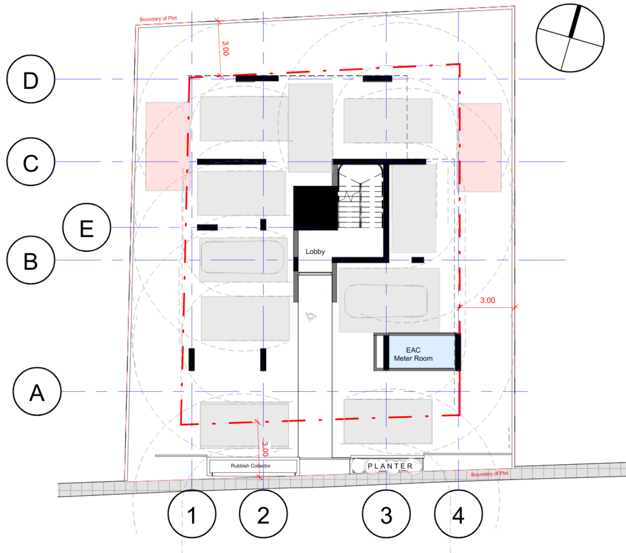
SIENA _Ground Floor
