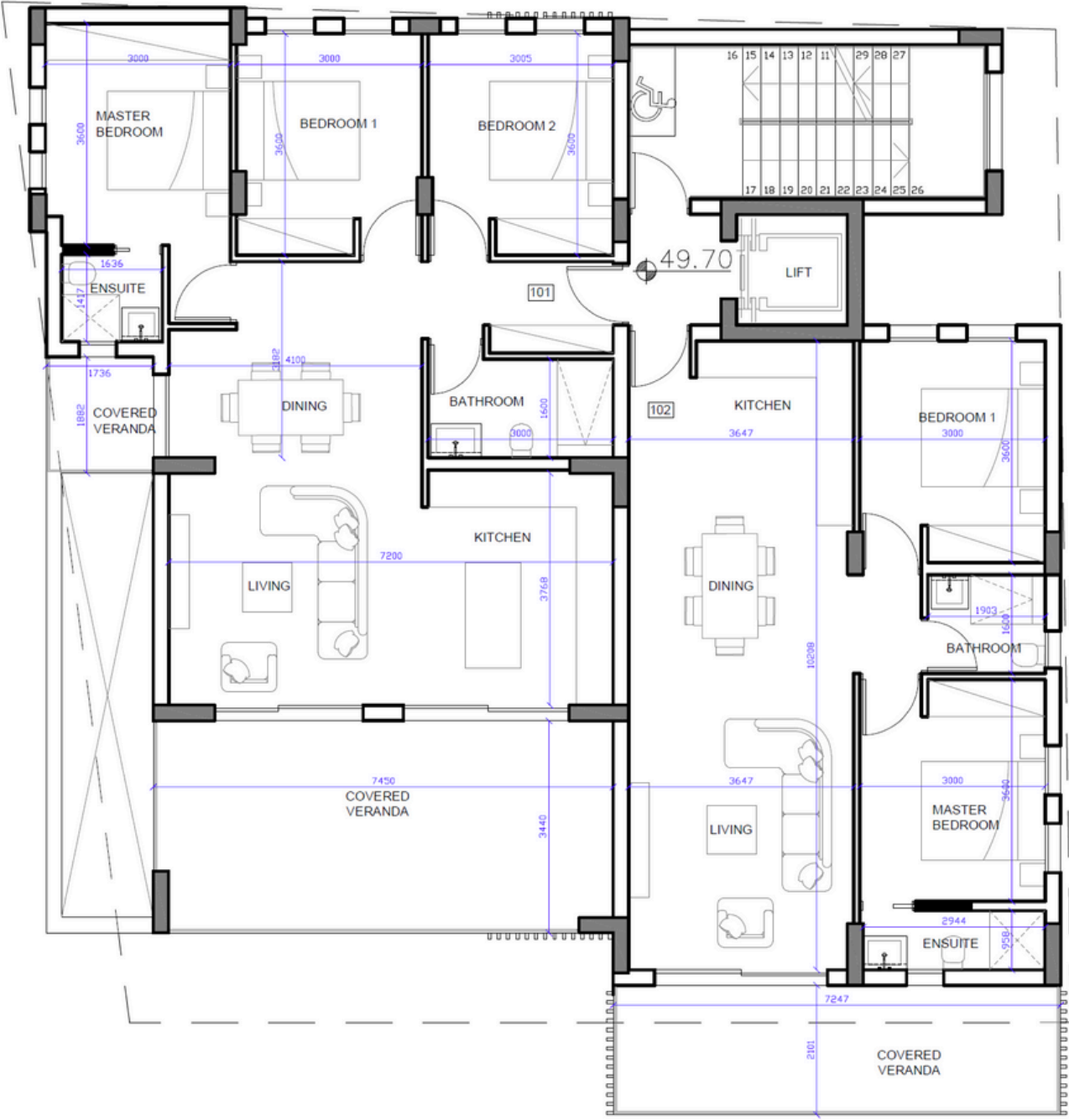
FIRST FLOOR
